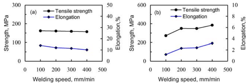
Figure 1 Tensile properties of the joints: (a) before heat treatment and (b) after heat treatment.
